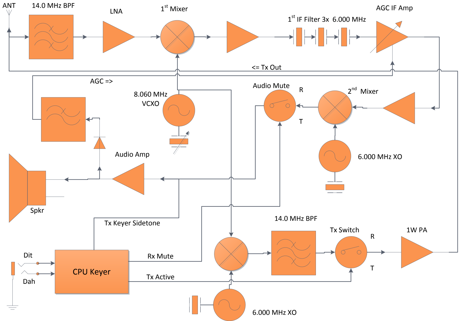
1Watter QRP Transceiver Block Diagram
